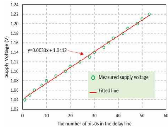
Fig. 3. Measured supply voltage represented by the number of bit-0s passing the delay line
