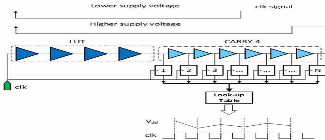
Fig. 1. Schematic of a supply voltage sensor
