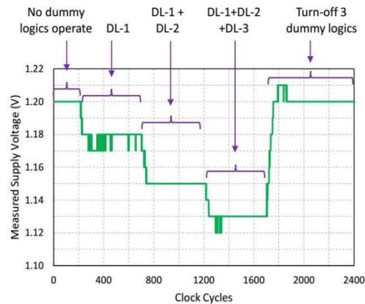
Fig. 5. Voltage drop measurement results
